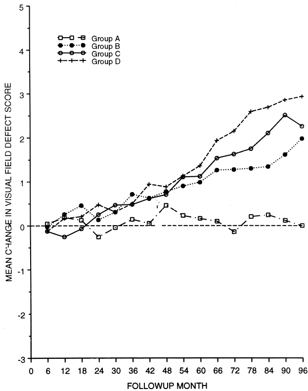
FIGURE 3. Associative Analysis. Mean change in visual field defect score by percent of visits over 6 years at which an eye presented with intraocular pressure less than 18 mm Hg (group A is 100%, group B is 75% to less than 100%, group C is 50% to less than 75%, and group D is 0% to less than 50%).
