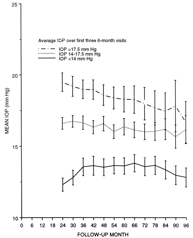
FIGURE 1. Predictive Analysis. Mean intraocular pressure ( \pm 2 SE) in the three intraocular pressure groups classified according to intraocular pressure averaged over the first three 6-month visits.
