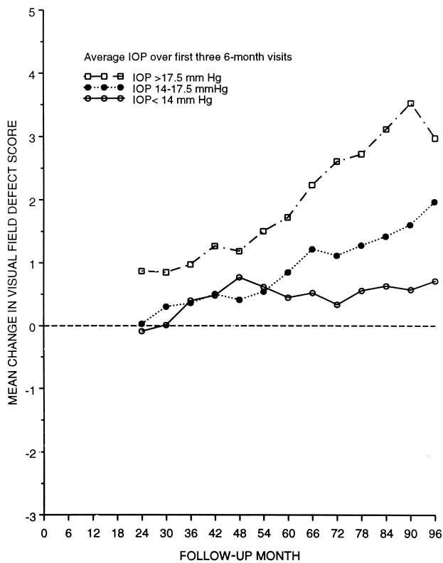
FIGURE 2. Predictive Analysis. Mean change from baseline in visual field defect score by intraocular pressure classified according to average value over the first three 6-month visits.
